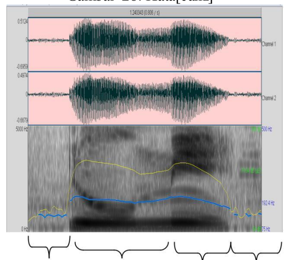
Gambar 28: Kata [cumi]
